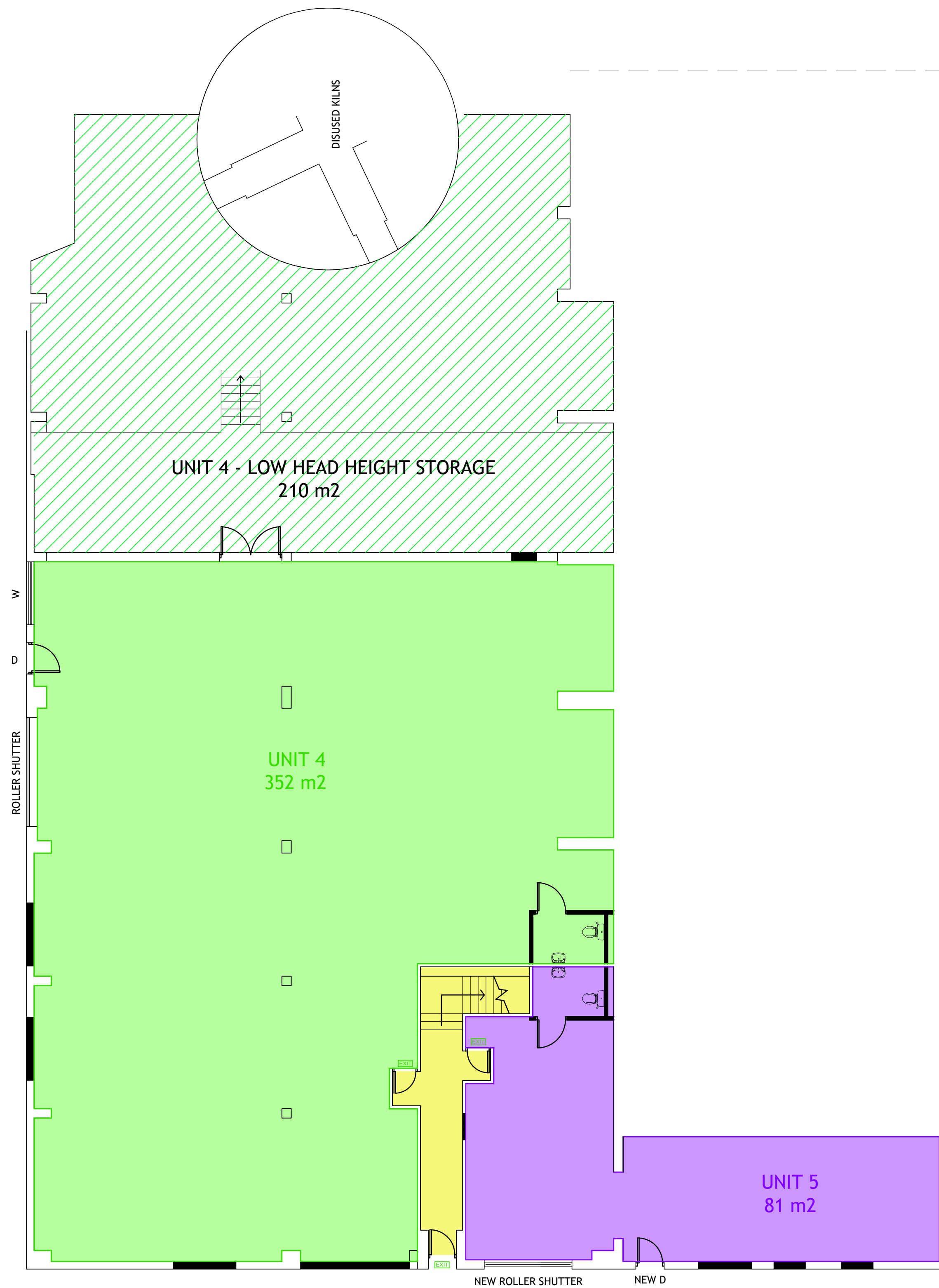
PROPOSED LOWER GROUND PLAN
